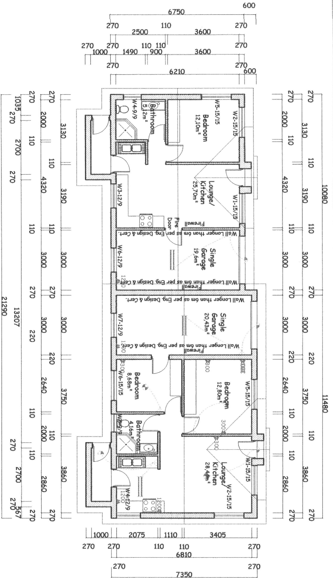
Typical 1 & 2 Bedroom Units 3,4,5 & 6 Ground Storey Floorplan Scale 1:100
